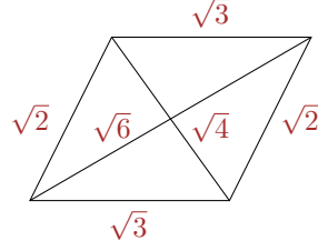
Figure II.1.3: Parallelogram with sides \sqrt{2} , \sqrt{3} and diagonals \sqrt{6} , \sqrt{4}
