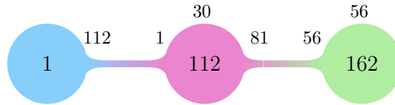
Figure II.1.7: The McLaughlin's graph
