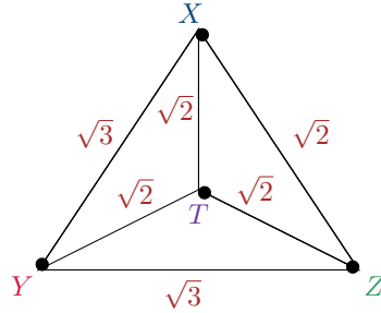
Figure II.1.4: Tetrahedra of type 332222
