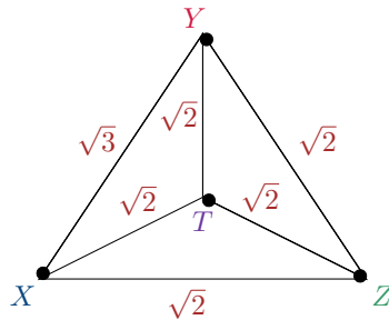
Figure II.1.6: Tetrahedra of type 322222
